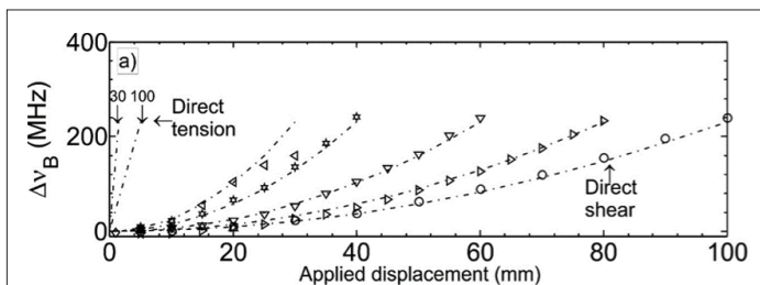
Figure 81: \Delta v_B changes in parabolic trend with shear displacement in comparison with the linear correlation from direct tension tests
