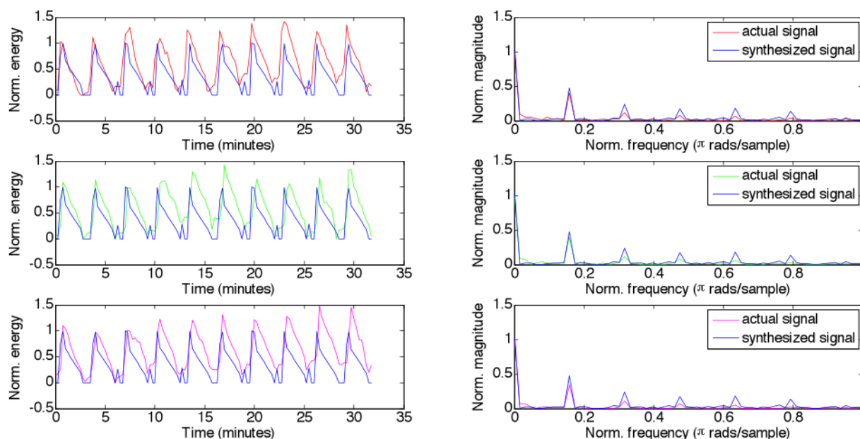
Figure 105: Identifying the 'fingerprint' of mine hoist operation within main mine electricity meter data, so that the hoist usage may be audited as part of a mine energy management plan. This technique is useful when only a single meter is installed at a mine site (which is frequently the case), and the usage of a particular centre of operations needs to be disaggregated for energy management
