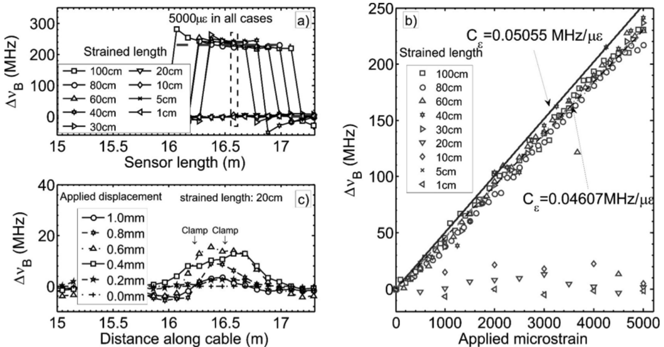
Figure 79: a) Brillouin frequency shift change ( \Delta\nu_B ) for application of 5000 \mu\epsilon to various strained lengths b) best-fit correlation between applied strain and \Delta\nu_B c) typical \Delta\nu_B response applying incremental displacement to a 20cm clamped length
