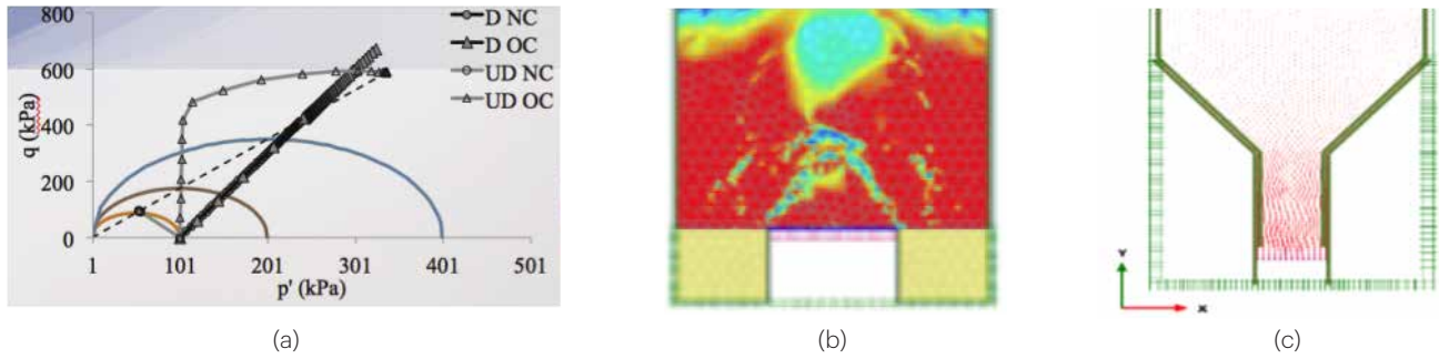
Figure 82: (a) Critical state concept in p' - q space; (b) trap door analogue for pillar loading showing strain localizations; and (c) silo analogue for drawpoints in caving operations
