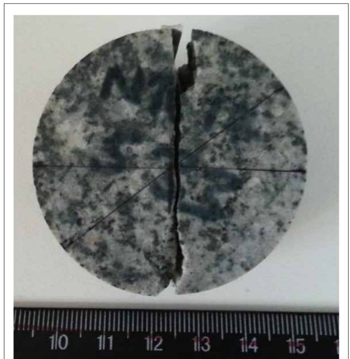
Figure 38: The Brazilian disc sample after the test with tensile failure along the line of loading
