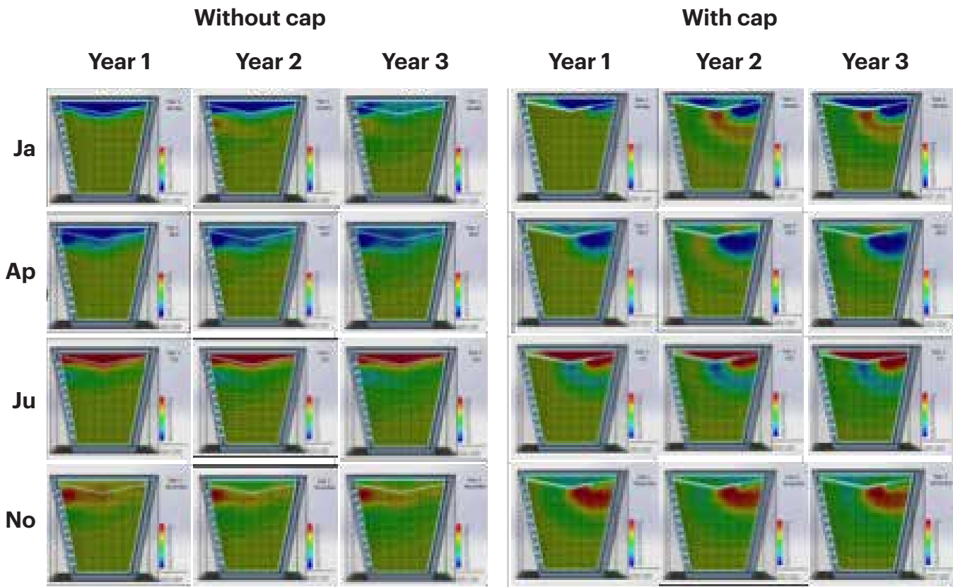
Figure: 99: Seasonal snapshots of the temperature field within a portion of fragmented rock 1/10th of the volume of Creighton Mine's NHEA. Air flow is from the top, horizontal surface to the steeply dipping LHS surface containing gaps denoting air flow control doors. LHS set (of 12) showing the seasonal temperature patterns when air flow can cross the whole of the top horizontal surface. RHS set (of 12) showing the seasonal temperature patterns when air flow can cross only the RHS of the top horizontal surface
