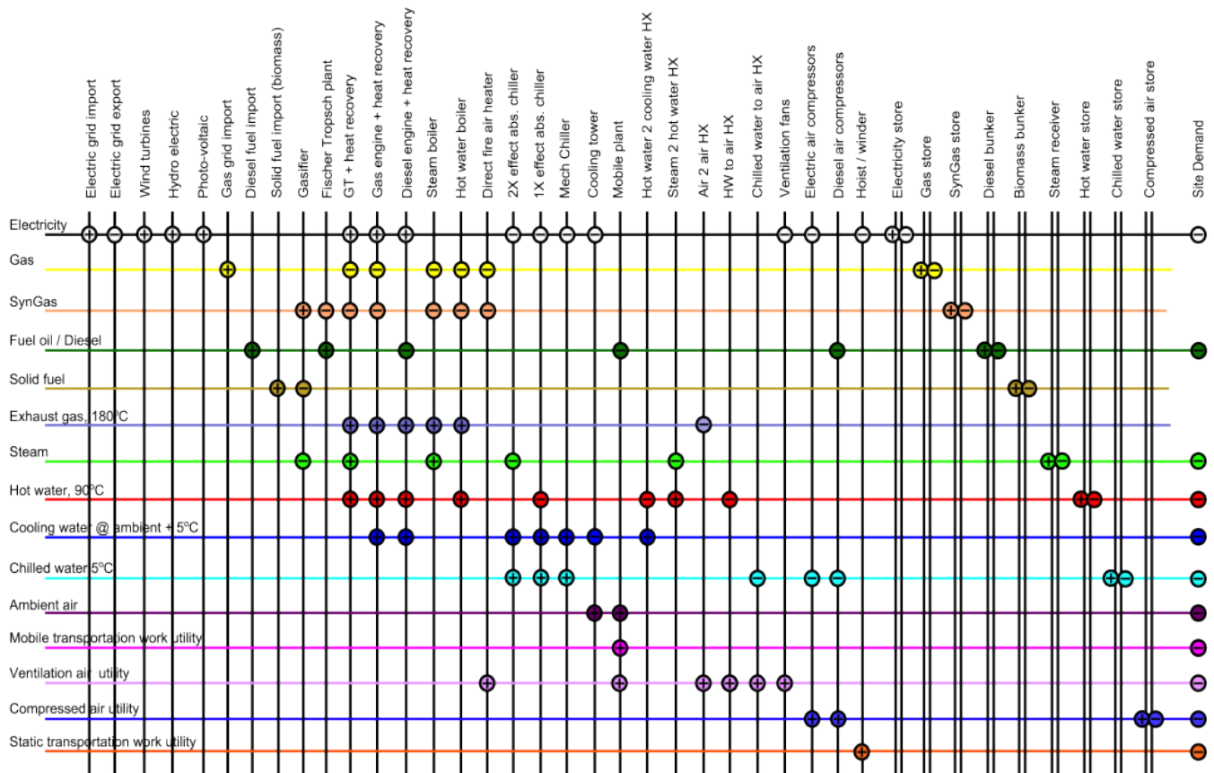
Figure 102: Conservative superstructural grid for an Optimal Mine Site Energy Supply problem involving 15 distinct types of energy supplied to a mine and 30 conventional and renewable energy conversion technologies with nine distinct types of energy storage technologies. Energy produced by a technology is denoted by a plus '+'. Energy consumed by a technology is denoted by a minus '-'. Consumption nodes on the extreme RHS denote the mine demand
