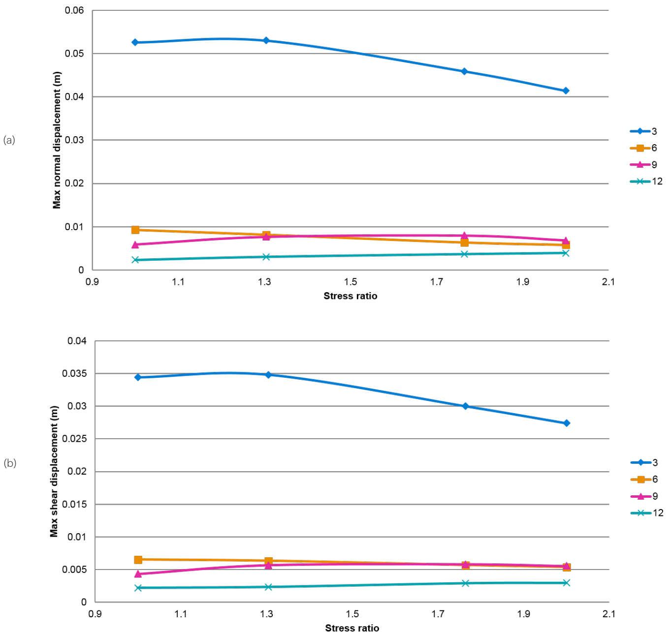
Figure 73: Maximum a) normal and b) shear displacements vs stress ratio for all injection points
