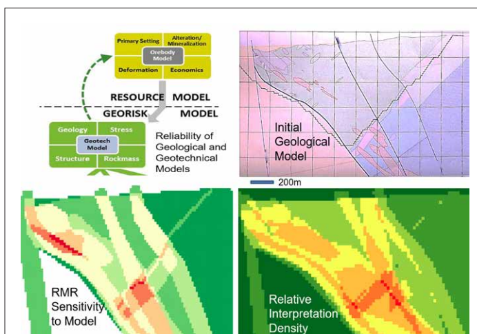
Figure 13: The geological model for an open pit and associated interpretation density (amount of geological input per volume) and geotechnical sensitivity (after O'Connor)
