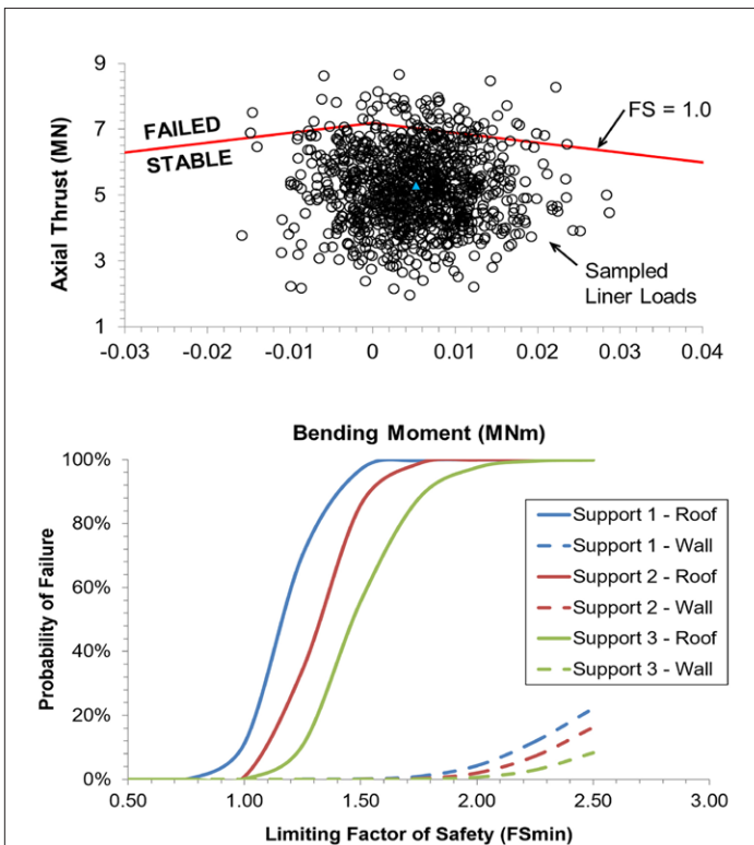
Figure 26: Example of rigorous reliability analysis for shotcrete rock support (Langford et al)
