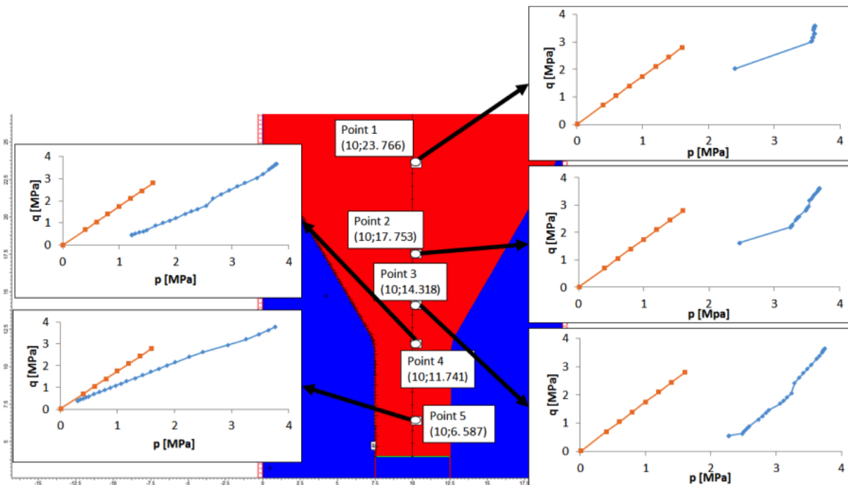
Figure 83: Stress path in mean stress p vs. deviator stress q space at five locations
