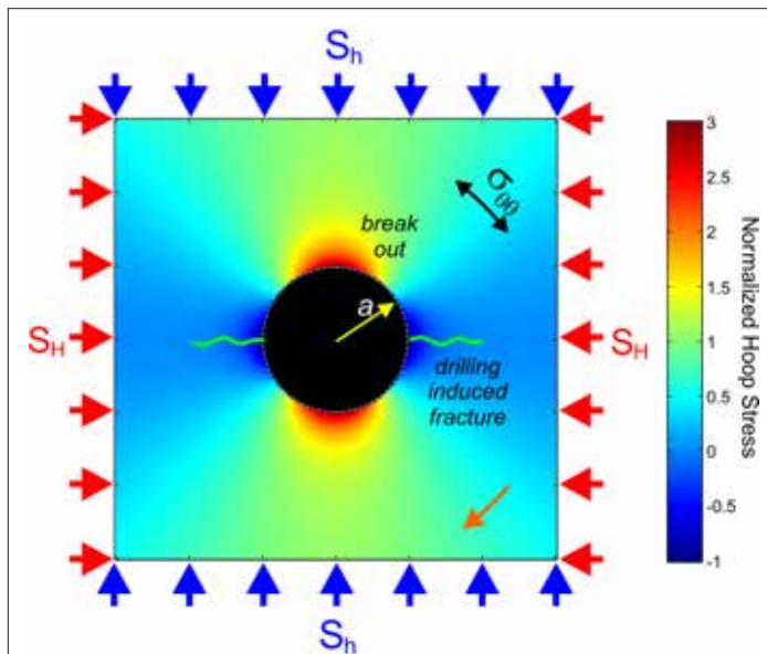
Figure 39: Illustration of the concentration of the azimuthal (hoop) stress by the borehole. Breakouts occur at the azimuth of the minimum horizontal compression S_{hmin} . Drilling-induced tensile fractures occur at the azimuth of the maximum horizontal compression S_{Hmax} .
