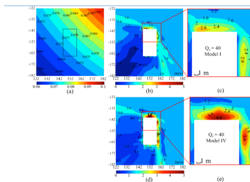
Site amplification of the slope. (a) PPV contour without excavation, which is based on the design scaling law with a 90-95% confidence level; (b) and (d) amplification factor contours around the slope and zoom-in plots (c) and (e) showing the detailed site amplification in the roof and on the right wall for uniform and non-uniform velocity models, respectively.
