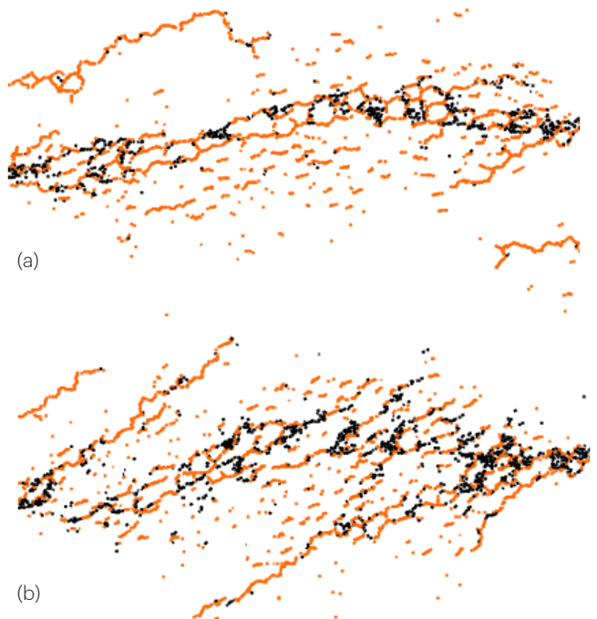
Figure 69: Shear rupture created in a soft, dilative environment under relatively low and high normal stress (Bewick et al., 2014)
